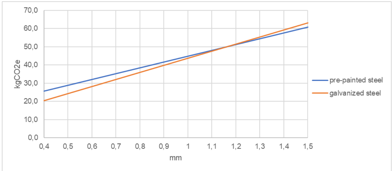
GWP-GHG variations with different steel thickness and finishes
